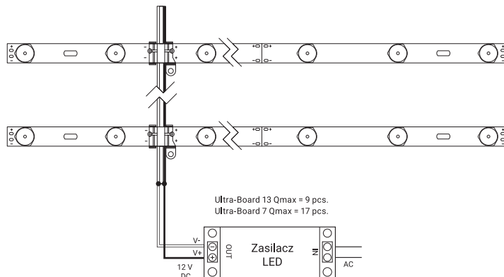
Fig. 1. Diagrams of the correct connection of the modules to the power supply.
