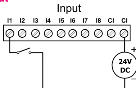
Picture 4 – Connection of input
