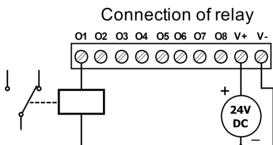
Picture 7 – Connection of relay
