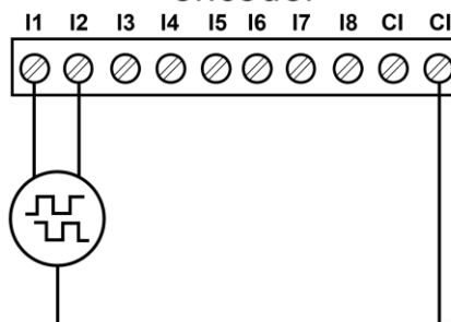
Picture 5 – Connection of encoder
