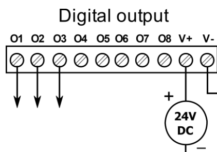
Picture 6 – Connection of digital output
