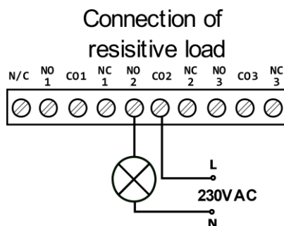
Picture 5- Connection of resistive load
