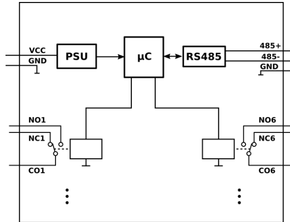
Picture 3- Block diagram
