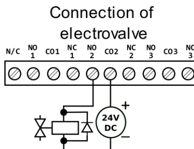
Picture 4- Connection of electrovalve
